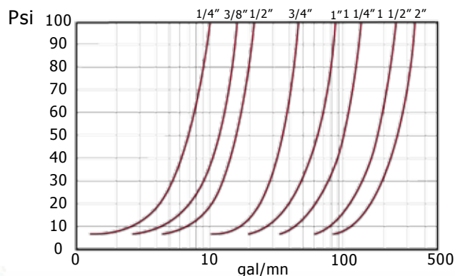
CHC Series Flow Chart
